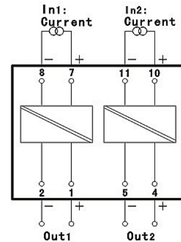
Basic Circuit Diagram UGLE-C/C-2/2
